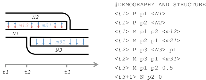
Figure 4. Illustration of the 'M' event type. In generation \langle t1 \rangle two subpopulations p1 and p2 are created. The migration rate is set to \langle m12 \rangle from p1 to p2 and \langle m21 \rangle in the other direction. In generation \langle t2 \rangle , subpopulation p3 splits off from p1 and migration from p1 to p3 is set to rate \langle m31 \rangle . In generation \langle t3 \rangle , subpopulation p2 admixes with subpopulation p1 , implemented by setting the fraction of p1 made up by migrants from p2 to 0.5 for that particular generation, and then eliminating p2 by setting its size to 0 in the following generation.
